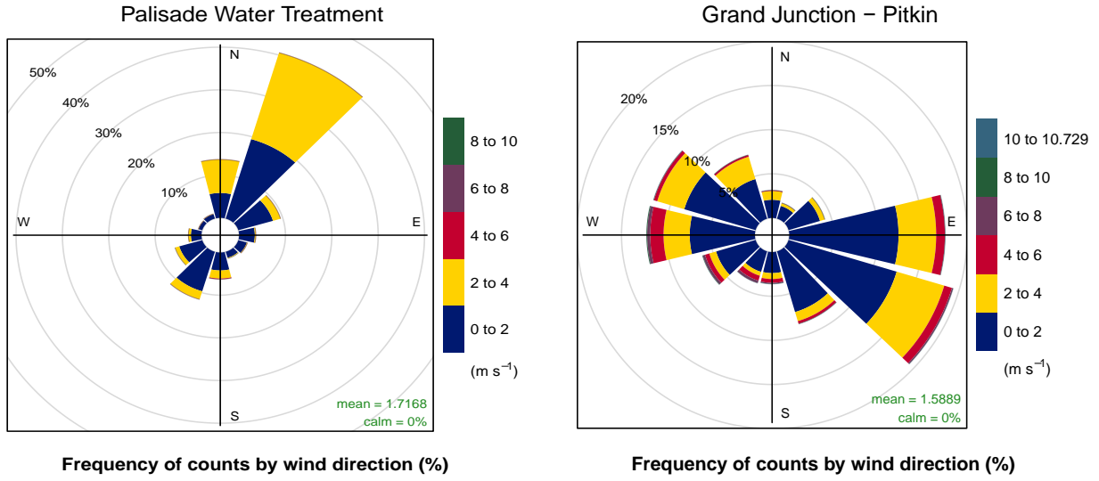
Figure 4.43: Wind roses for sites in the Western Slope Region during 2022.
