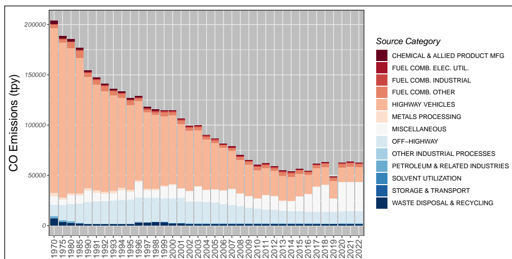
Figure 2.1: Trends in national carbon monoxide emissions from 1970 to 2022.
