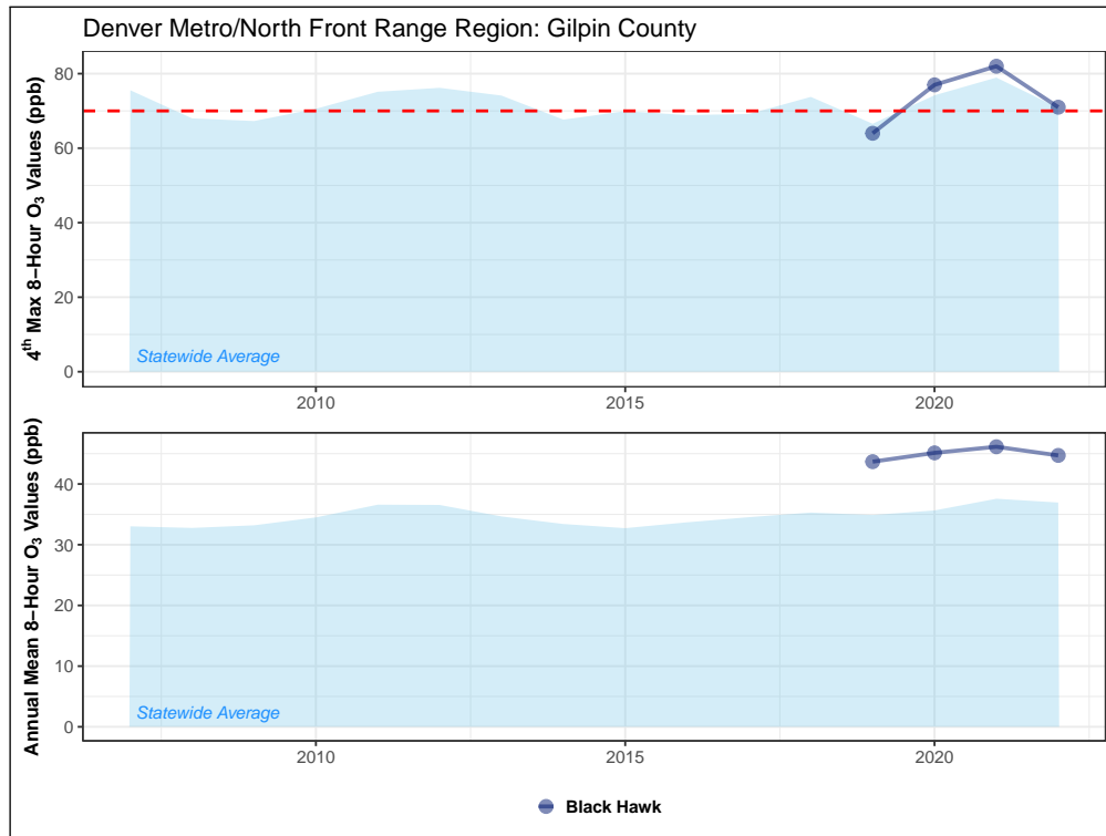
Figure 4.16: Fifteen-year trend in ozone eight-hour NAAQS values (top) and annual mean eight-hour concentrations (bottom) for monitoring sites in Gilpin County. The eight-hour NAAQS (70 ppb) is shown as a dashed red line.
