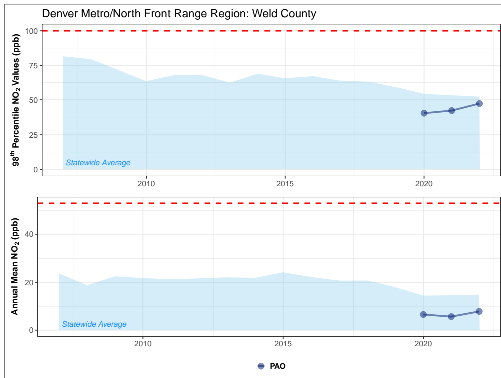
Figure 4.23: Fifteen-year trend in one-hour (top) and annual mean (bottom) nitrogen dioxide NAAQS values for monitoring sites in Weld County. The one-hour and annual mean standards (100 ppb and 53 ppb, respectively) are shown as dashed red lines.
