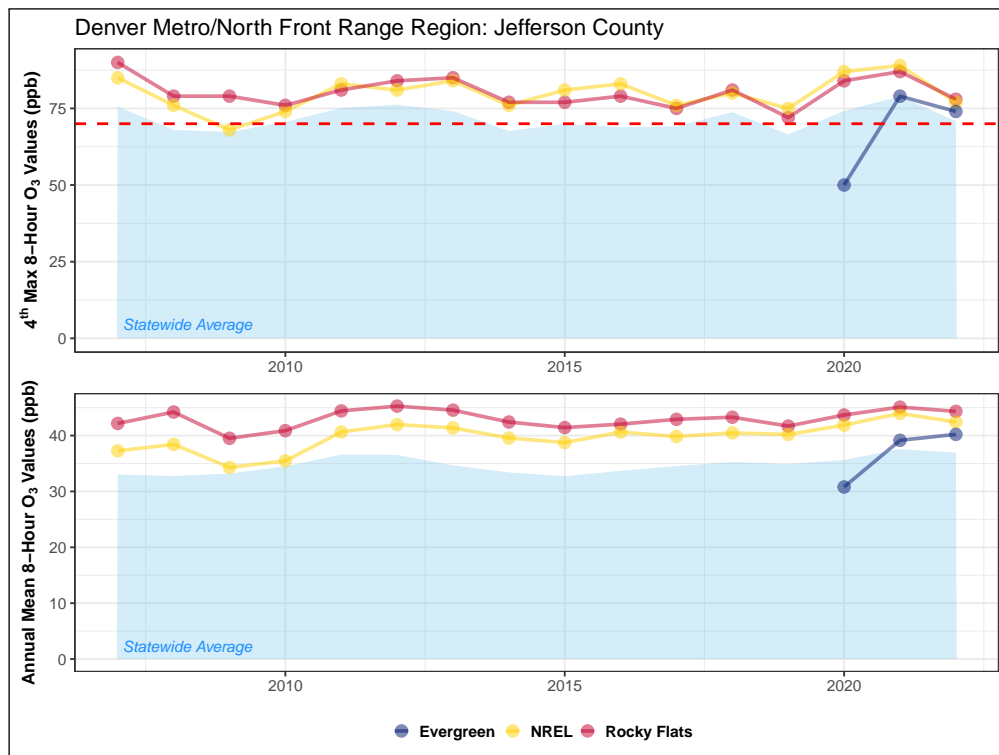
Figure 4.17: Fifteen-year trend in ozone eight-hour NAAQS values (top) and annual mean eight-hour concentrations (bottom) for monitoring sites in Jefferson County. The eight-hour NAAQS (70 ppb) is shown as a dashed red line.
