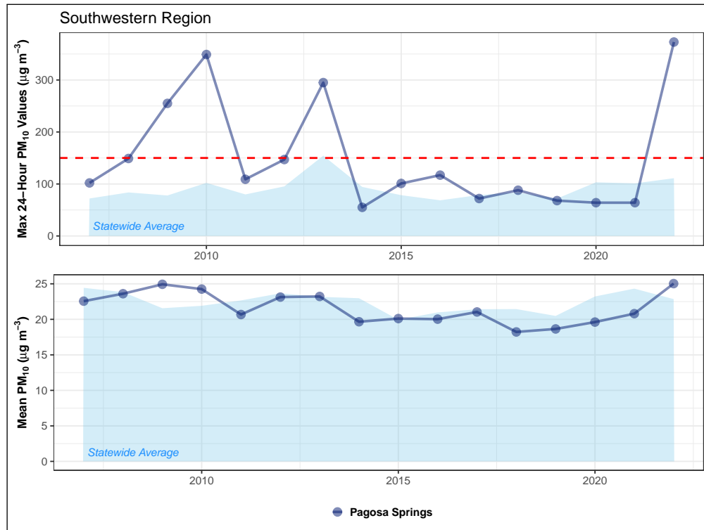
Figure 4.38: Fifteen-year trend in maximum 24-hour PM 10 values (top) and annual mean concentrations (bottom) for monitoring sites in the Southwest region. The 24-hour NAAQS (150 µg m -3 ) is shown as a dashed red line.
