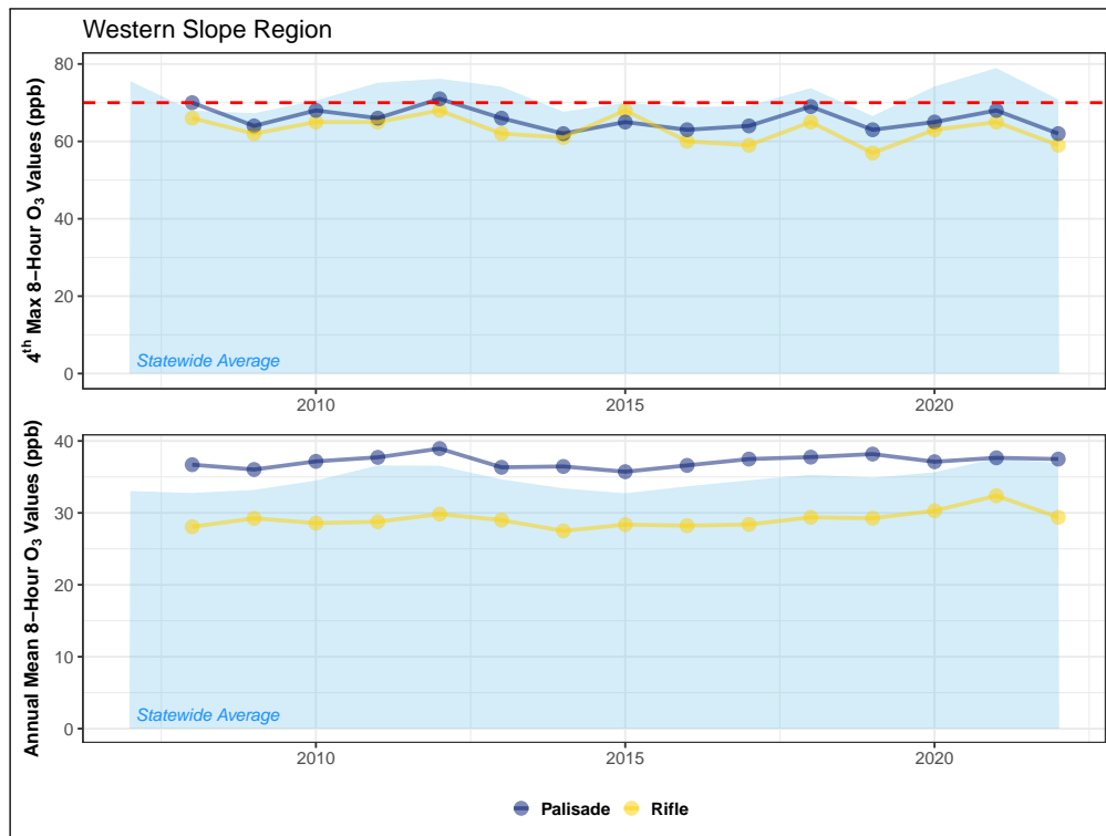
Figure 4.42: Fifteen-year trend in ozone eight-hour NAAQS values (top) and annual mean eight-hour concentrations (bottom) for monitoring sites in the Western Slope region. The eight-hour NAAQS (70 ppb) is shown as a dashed red line.
