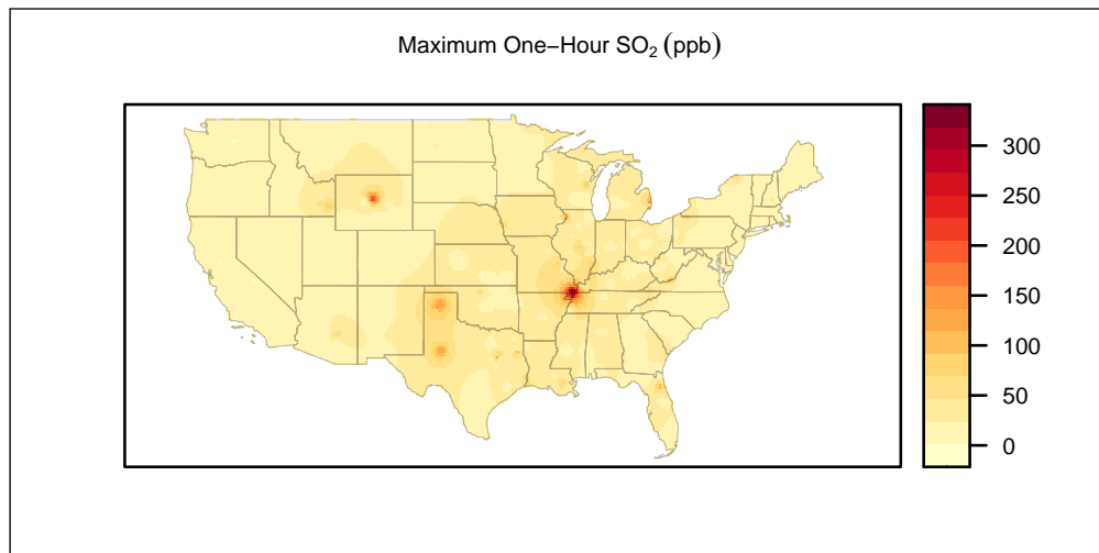
Figure 2.9: Interpolation map of maximum one-hour SO 2 values for air quality monitoring stations in the continental U.S. during 2022
