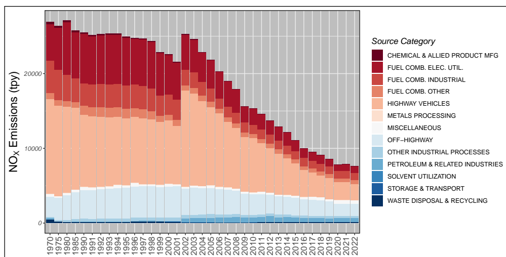
Figure 2.13: Trends in national NO x emissions from 1970 to 2022.
