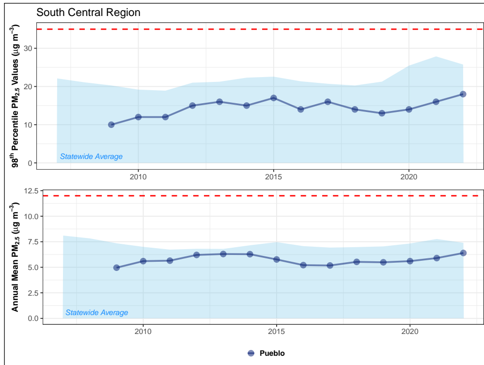
Figure 4.37: Fifteen-year trend in 24-hour PM 2.5 annual 98 th percentile values (top) and annual mean concentrations (bottom) for monitoring sites in the South Central region. The 24-hour and annual mean NAAQS (35 µg m -3 and 12 µg m -3 , respectively) are shown as dashed red lines.
