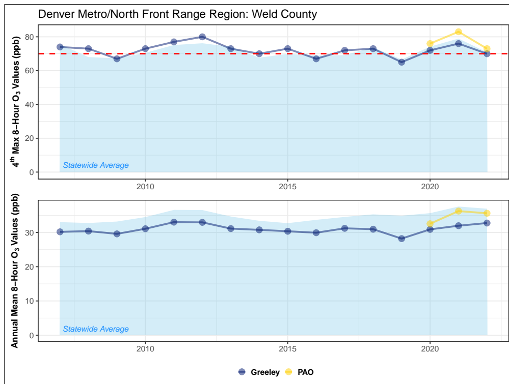
Figure 4.19: Fifteen-year trend in ozone eight-hour NAAQS values (top) and annual mean eight-hour concentrations (bottom) for monitoring sites in Weld County. The eight-hour NAAQS (70 ppb) is shown as a dashed red line.
