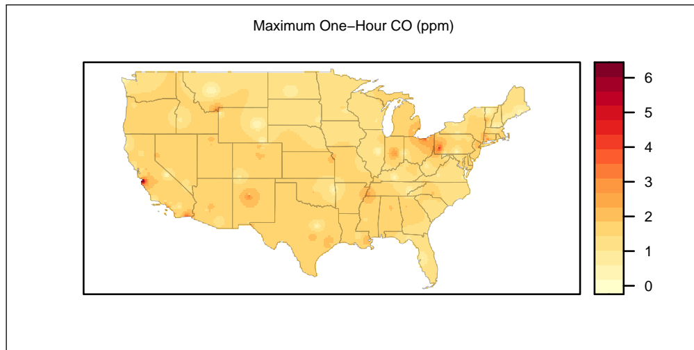
Figure 2.5: Interpolation map of maximum one-hour CO values for air quality monitoring stations in the continental U.S. during 2022
