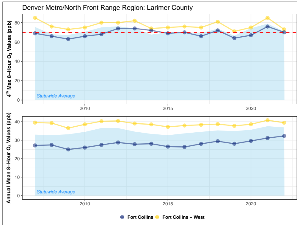
Figure 4.18: Fifteen-year trend in ozone eight-hour NAAQS values (top) and annual mean eight-hour concentrations (bottom) for monitoring sites in Larimer County. The eight-hour NAAQS (70 ppb) is shown as a dashed red line.
