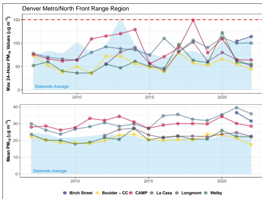
Figure 4.2: Fifteen-year trend in maximum 24-hour PM 10 values (top) and annual mean concentrations (bottom) for monitoring sites in the Denver Metro/Northern Front Range region. The 24-hour NAAQS (150 µg m -3 ) is shown as a dashed red line.
