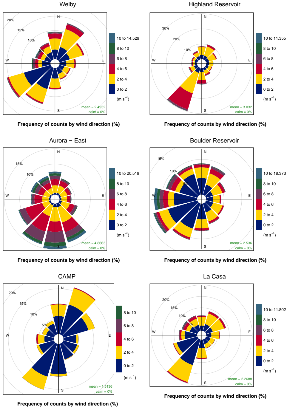
Figure 4.26: Wind roses for sites in the Denver Metro/North Front Range Region during 2022.
