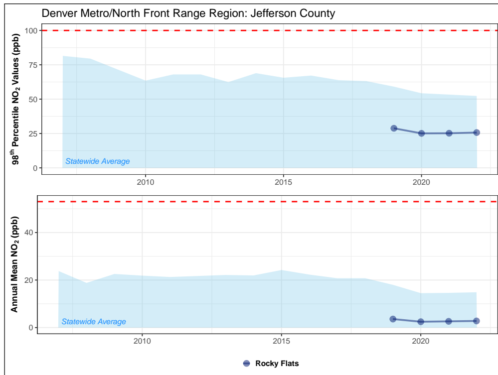
Figure 4.22: Fifteen-year trend in one-hour (top) and annual mean (bottom) nitrogen dioxide NAAQS values for monitoring sites in Jefferson County. The one-hour and annual mean standards (100 ppb and 53 ppb, respectively) are shown as dashed red lines.
