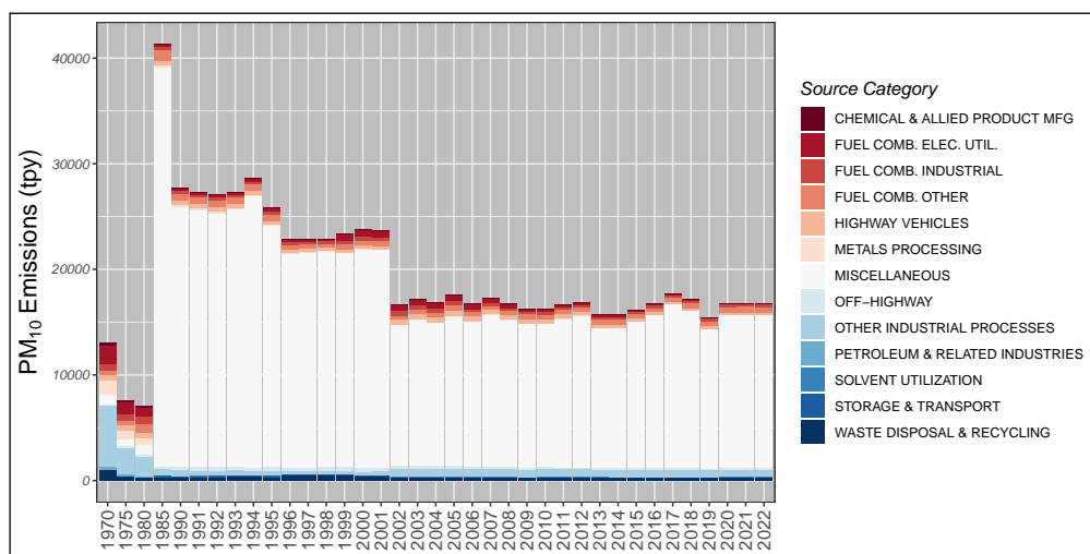
Figure 2.18: Trends in national \text{PM}_{10} emissions from 1970 to 2022.
