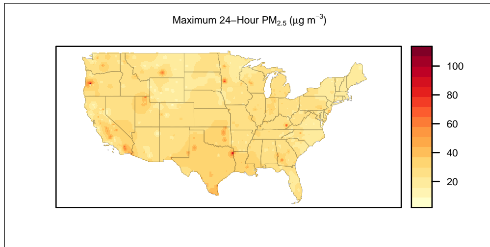
Figure 2.24: Interpolation map of maximum 24-hour PM 2.5 values for air quality monitoring stations in the continental U.S. during 2022
