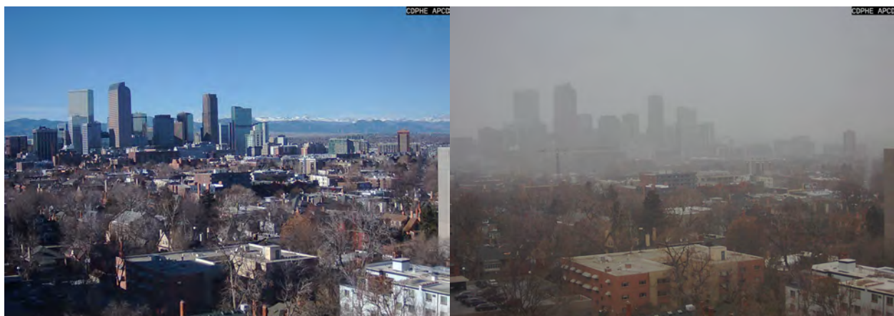
Figure 3.3: Denver Camera images of the best (left) and worst (right) visibility days in Denver during 2022.
