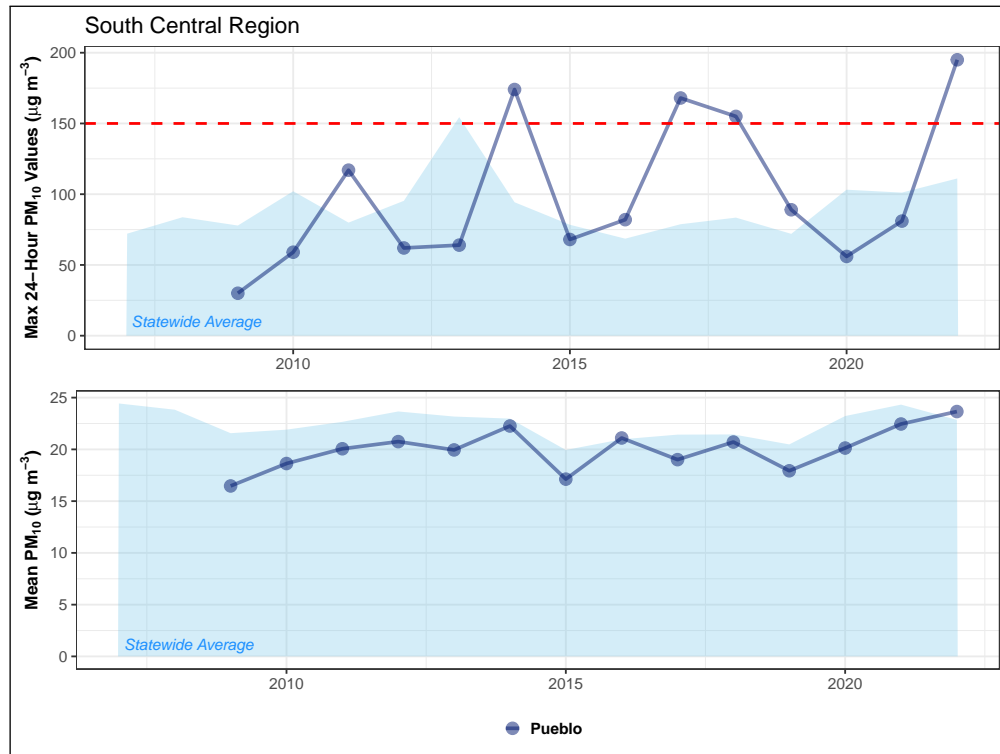
Figure 4.36: Fifteen-year trend in maximum 24-hour PM 10 values (top) and annual mean concentrations (bottom) for monitoring sites in the South Central region. The 24-hour NAAQS (150 µg m -3 ) is shown as a dashed red line.
