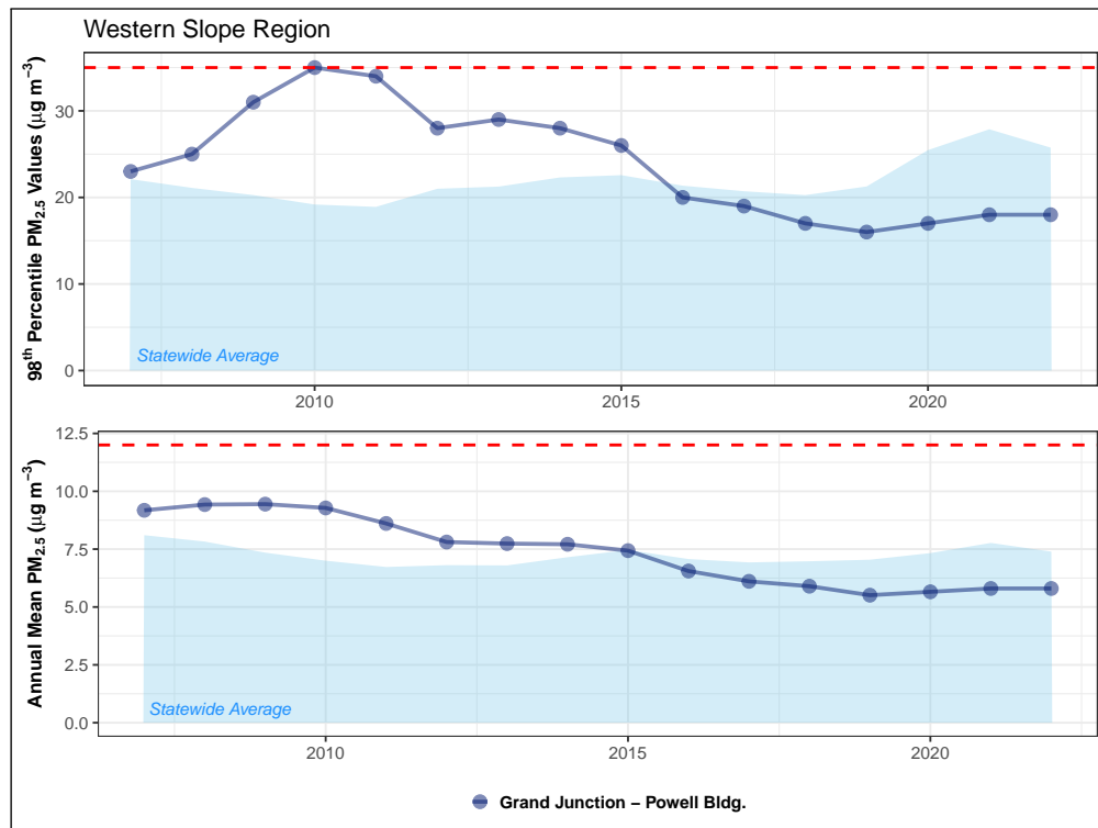
Figure 4.41: Fifteen-year trend in 24-hour PM 2.5 annual 98 th percentile values (top) and annual mean concentrations (bottom) for monitoring sites in the Western Slope region. The 24-hour and annual mean NAAQS (35 µg m -3 and 12 µg m -3 , respectively) are shown as dashed red lines.
