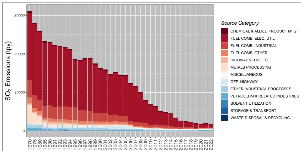
Figure 2.6: Trends in national sulfur dioxide emissions from 1970 to 2022.
