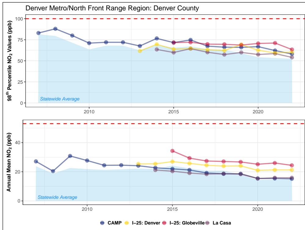
Figure 4.21: Fifteen-year trend in one-hour (top) and annual mean (bottom) nitrogen dioxide NAAQS values for monitoring sites in Denver County. The one-hour and annual mean standards (100 ppb and 53 ppb, respectively) are shown as dashed red lines.
