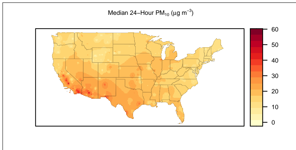
Figure 2.21: Interpolation map of median 24-hour PM 10 values for air quality monitoring stations in the continental U.S. during 2022
