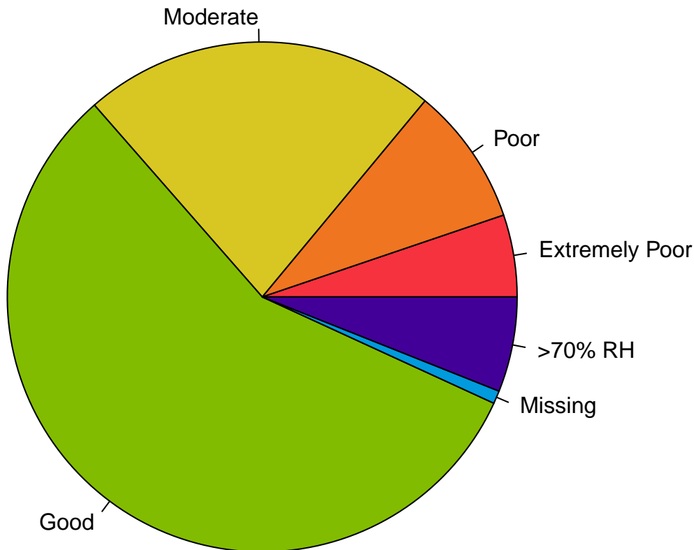
Figure 4.25: Denver visibility data.
