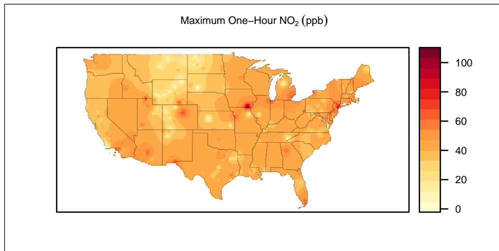
Figure 2.17: Interpolation map of maximum one-hour NO 2 values for air quality monitoring stations in the continental U.S. during 2022
