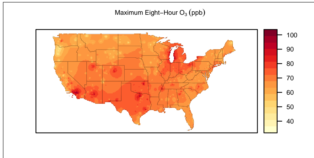
Figure 2.12: Interpolation map of maximum eight-hour O 3 values for air quality monitoring stations in the continental U.S. during 2022
