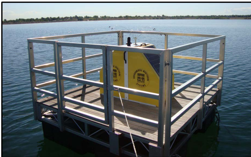
Figure 3. Water-Quality Profiler at SL10
