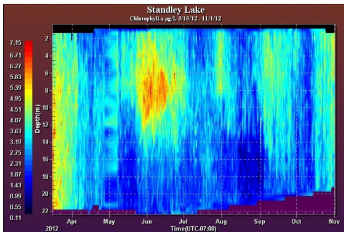
Figure 66. Isopleth of Chlorophyll a Concentrations in Standley Lake, March-October 2012
