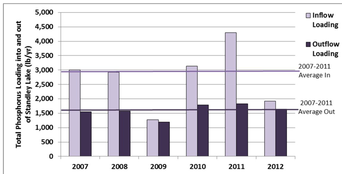
Figure ES-6. Total Phosphorus Loading into and out of Standley Lake, using Grab Samples and 24-Hour Ambient Autosampler Data, 2007-2012
