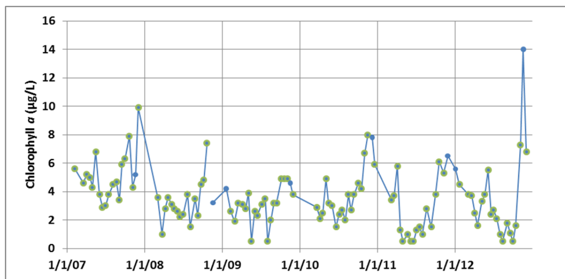
Figure 64. Chlorophyll a Concentrations in Standley Lake, 2007-2012 (with March-November observations highlighted)
