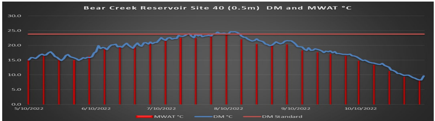
Figure 41 Temperature Compliance Bear Creek Reservoir
