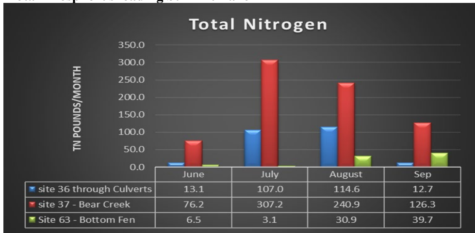
Figure 38 Total Nitrogen Loading Summit Lake
