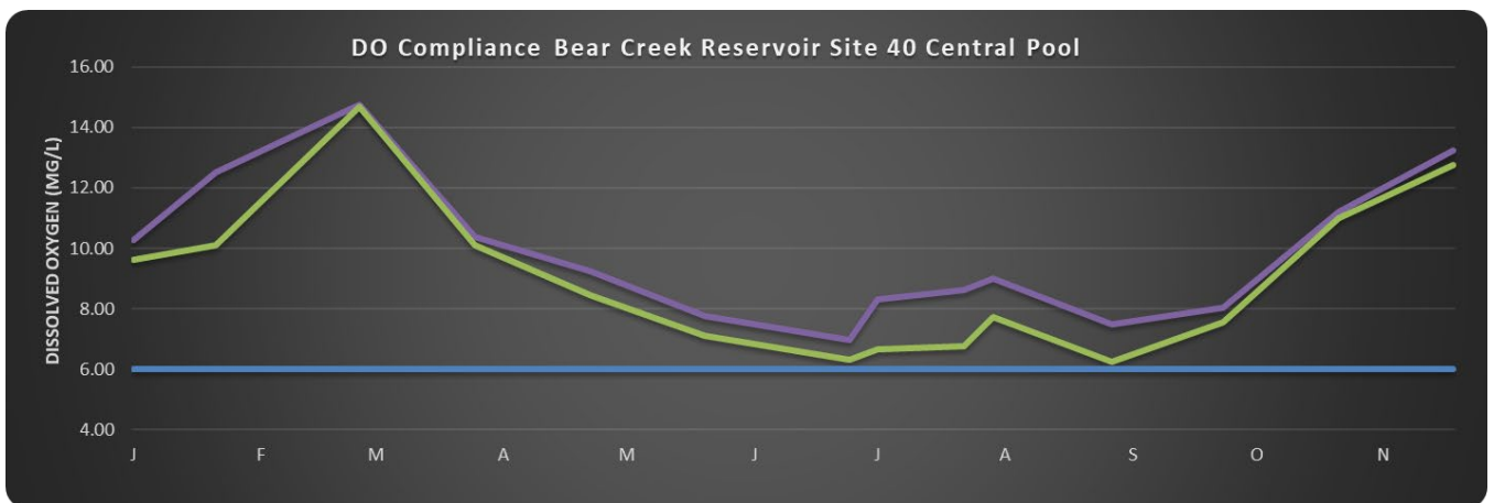
Figure 10 Dissolved Oxygen Compliance in Bear Creek Reservoir
