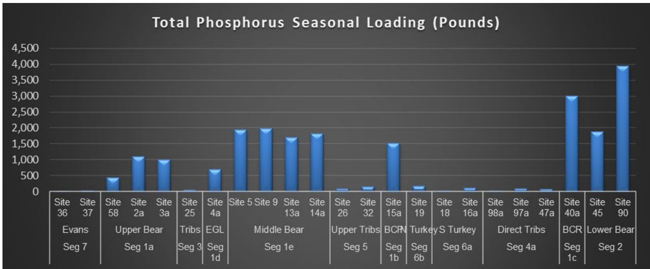
Figure 6 Total Phosphorus Loading (pounds) by Stream Segment in the Watershed
