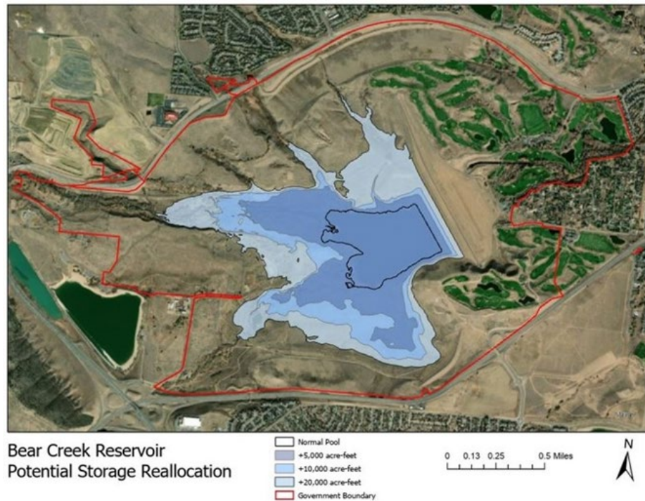
Figure 42 Potential BCR Reallocation
