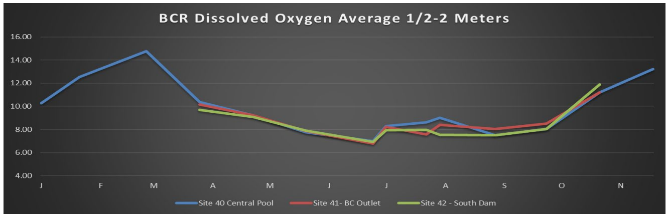
Figure 27 Bear Creek Reservoir 2021 Dissolved Oxygen Trend
