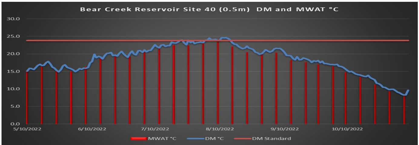
Figure 9 Bear Creek Reservoir Daily Maximum Temperatures at Site 40(0.5m)
