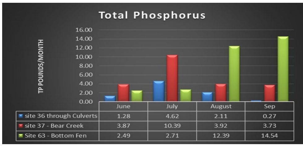
Figure 37 Total Phosphorus loading Summit Lake
