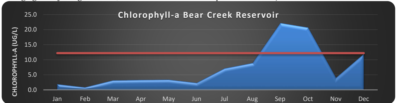
Figure 23 Bear Creek Reservoir Chlorophyll Trend
