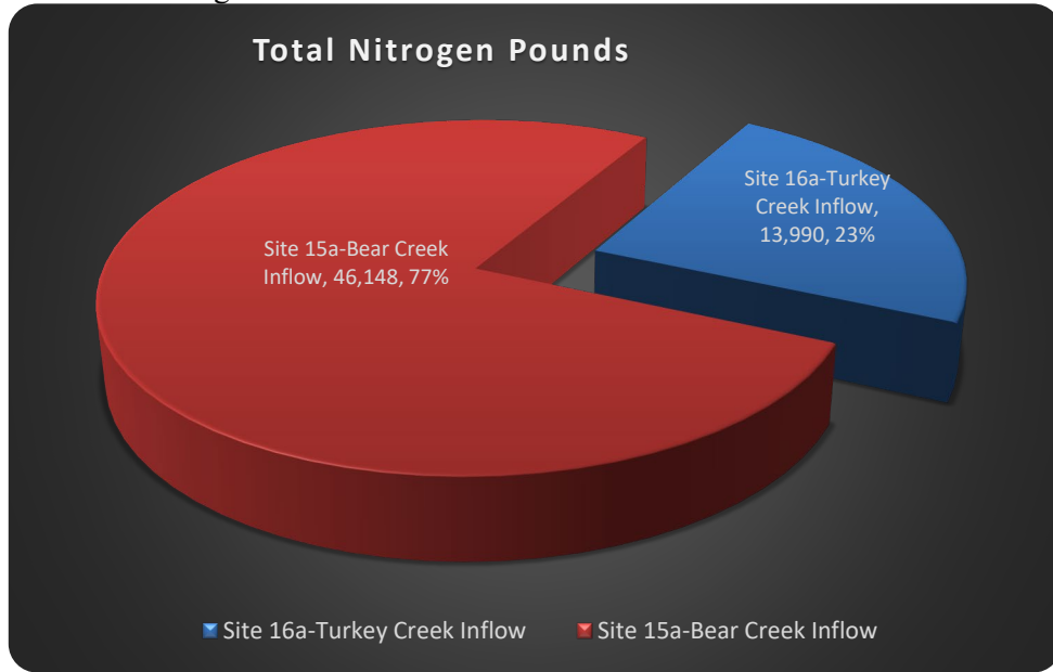
Figure 20 Total Nitrogen Loading into Bear Creek Reservoir
