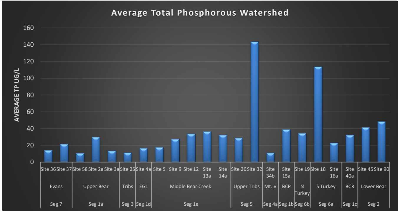
Figure 3 Total Phosphorus Concentrations by Stream Segments in the Watershed
