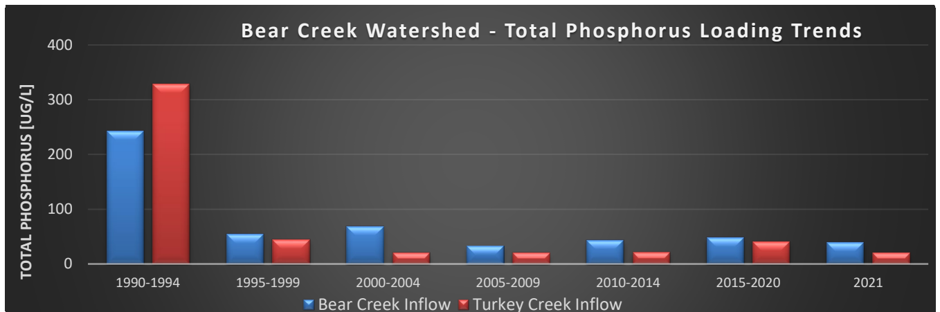
Figure 19 5-Year Average Total Phosphorus Trend BCR Compared with 2021
