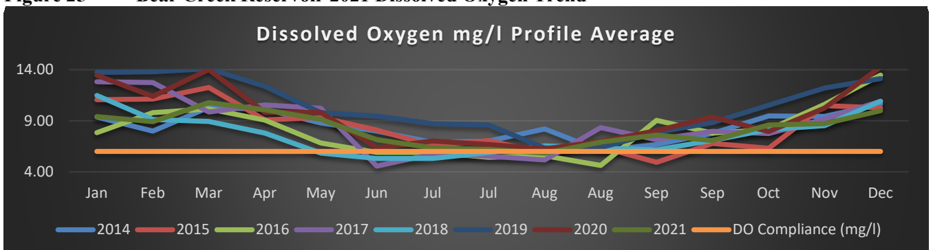
Figure 26 Dissolved Oxygen Trend 2014-2021
