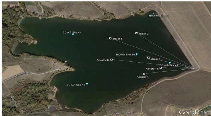
Figure 27 BCR Aeration Configuration
