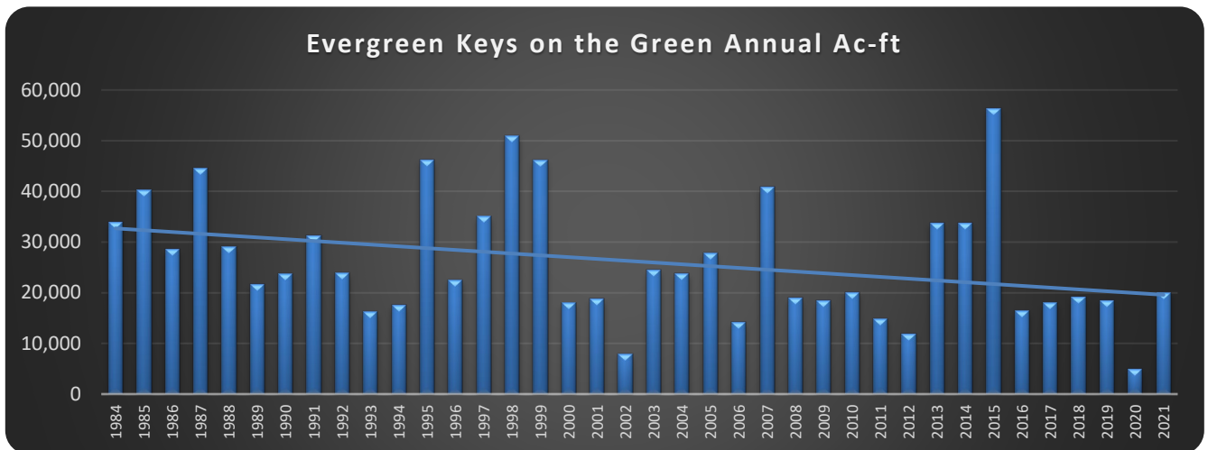
Figure 17 Bear Creek at Keys-on-the-Green, above Evergreen
