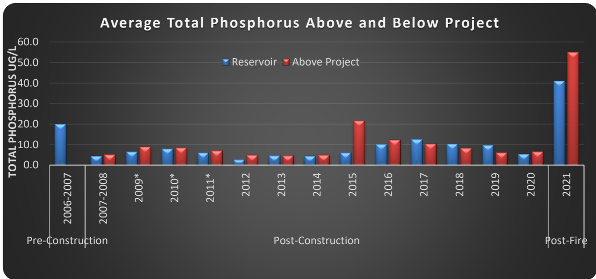
Figure 9 Total Phosphorus Reduction at Coyote Gulch Restoration Site
