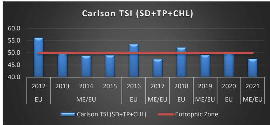
Figure 29 Trophic State of Evergreen Lake using Carlson Index
