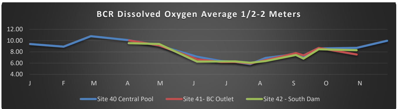
Figure 25 Bear Creek Reservoir 2021 Dissolved Oxygen Trend
