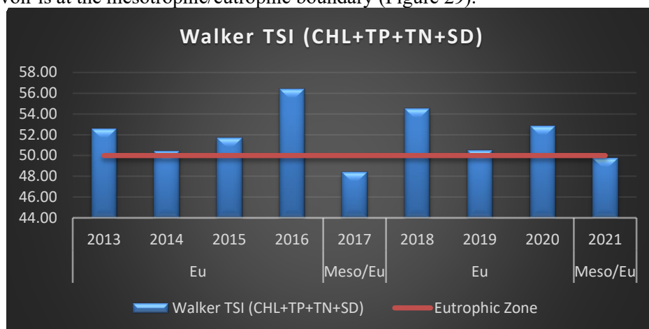
Figure 28 Trophic State of Evergreen Lake using Walker Index
