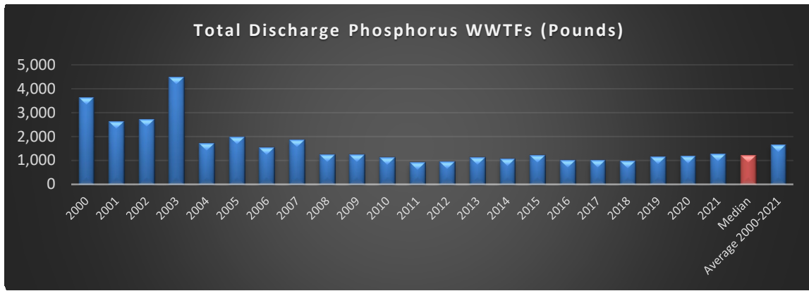
Figure 6 Point Source Load Reaching Bear Creek Reservoir
