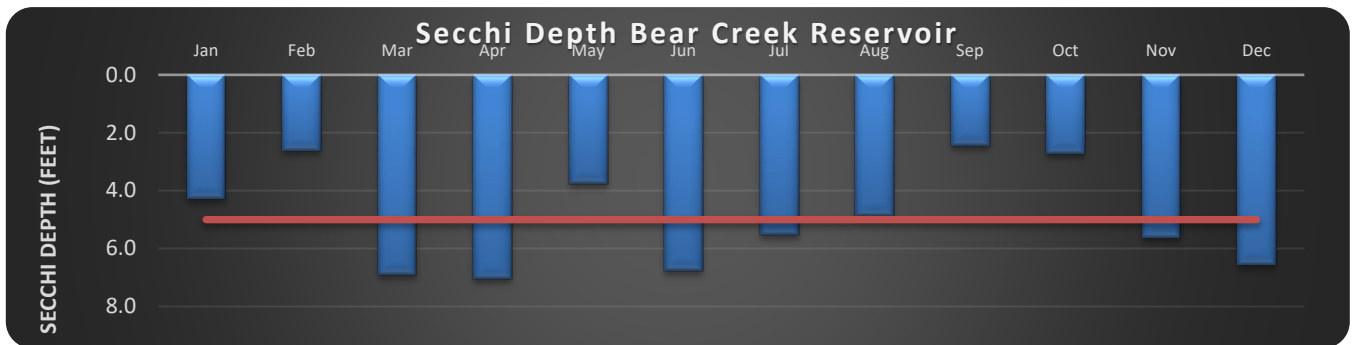
Figure 22 Secchi Depth Bear Creek Reservoir
