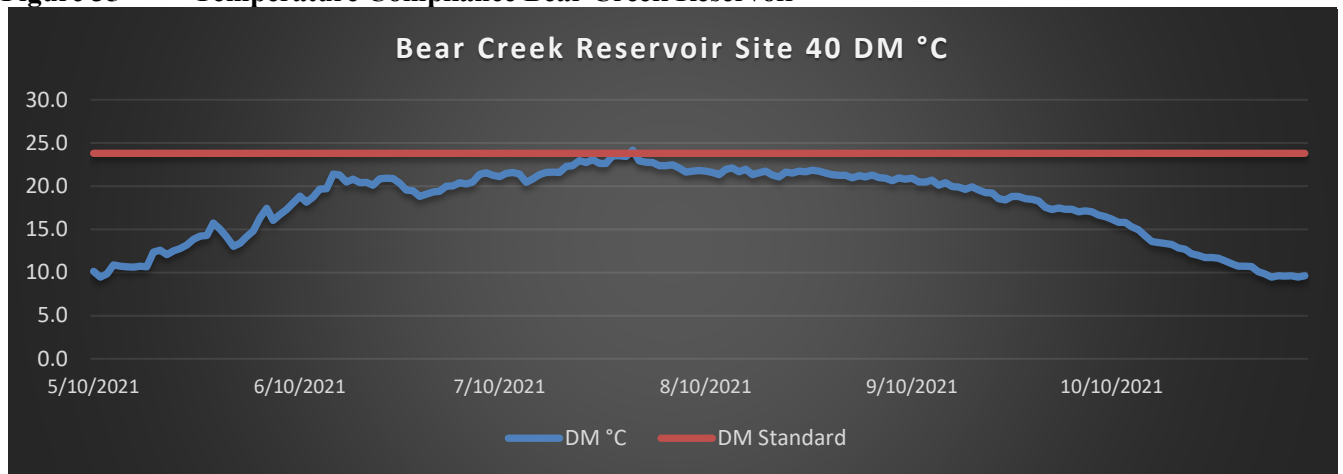
Figure 36 Daily Maximum Temperature Probe Record BCR
