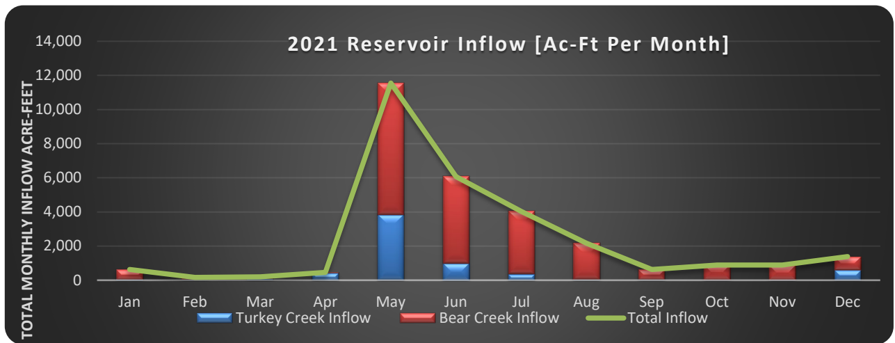
Figure 13 In-Flow Estimates by Month into Bear Creek Reservoir
