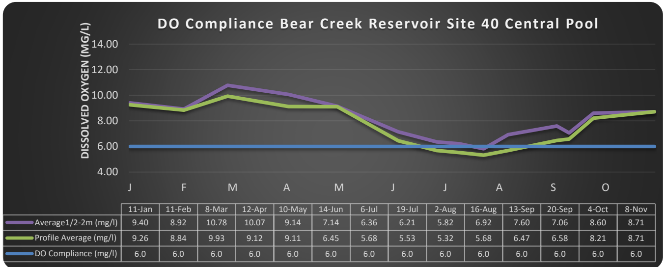
Figure 34 DO Compliance Bear Creek Reservoir
