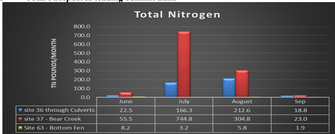
Figure 32 Total Nitrogen Loading Summit Lake
