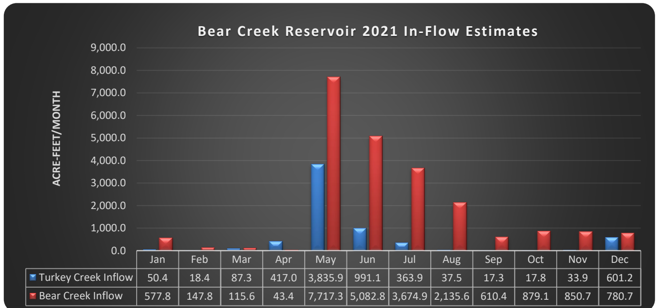
Figure 15 Annual Flows into Bear Creek Reservoir
