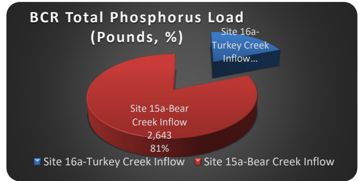
Figure 18 Estimated Total Phosphorus loading into Bear Creek Reservoir
