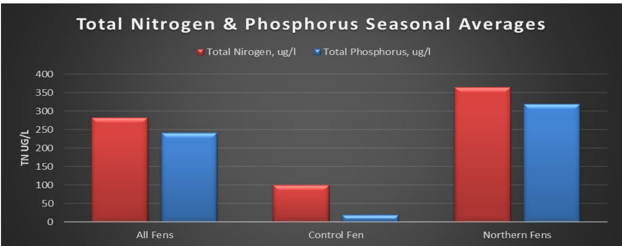
Figure 33 Total Phosphorus and Total Nitrogen Seasonal Averages in Fen Complex
