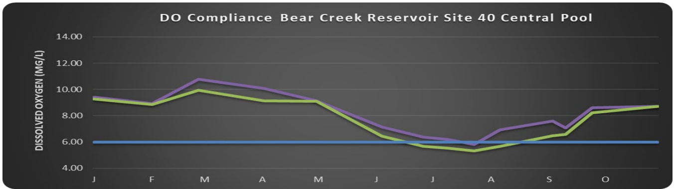
Figure 8 Dissolved Oxygen Compliance in Bear Creek Reservoir
