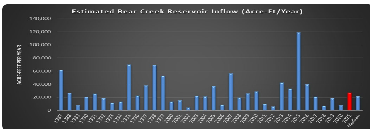
Figure 1 Estimated Bear Creek Reservoir Inflow 1987-2021
