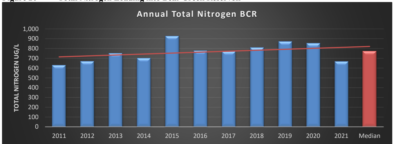
Figure 21 Estimated Total Nitrogen Loading Trend for Bear Creek Reservoir
