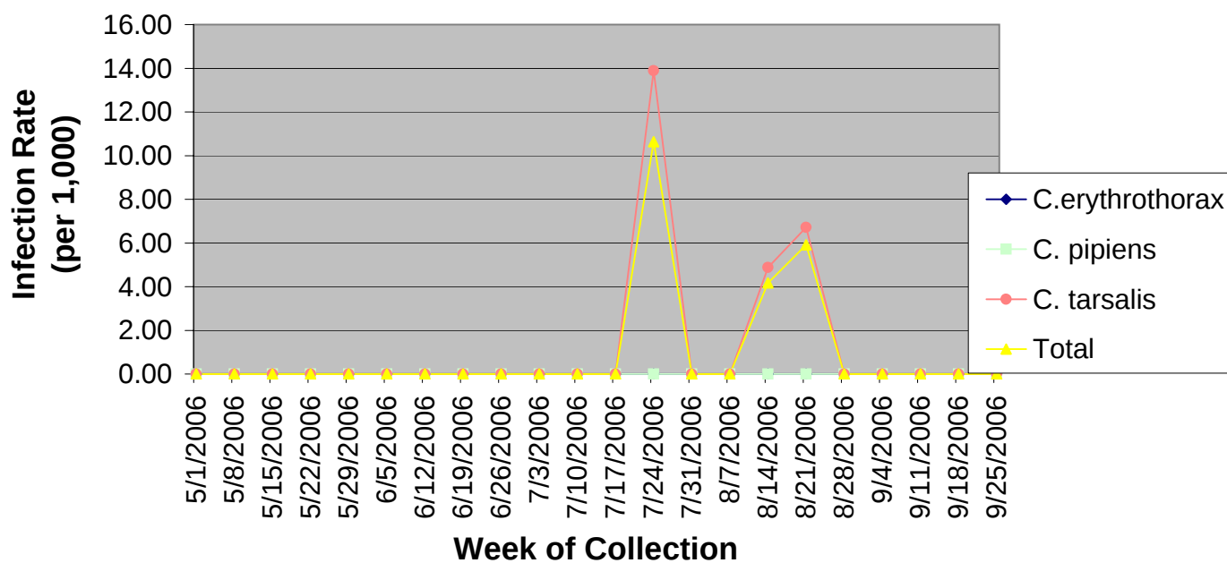
Mosquito Minimum WNV Infection Rates, Culex Species Larimer County Sentinel Site, 2006
