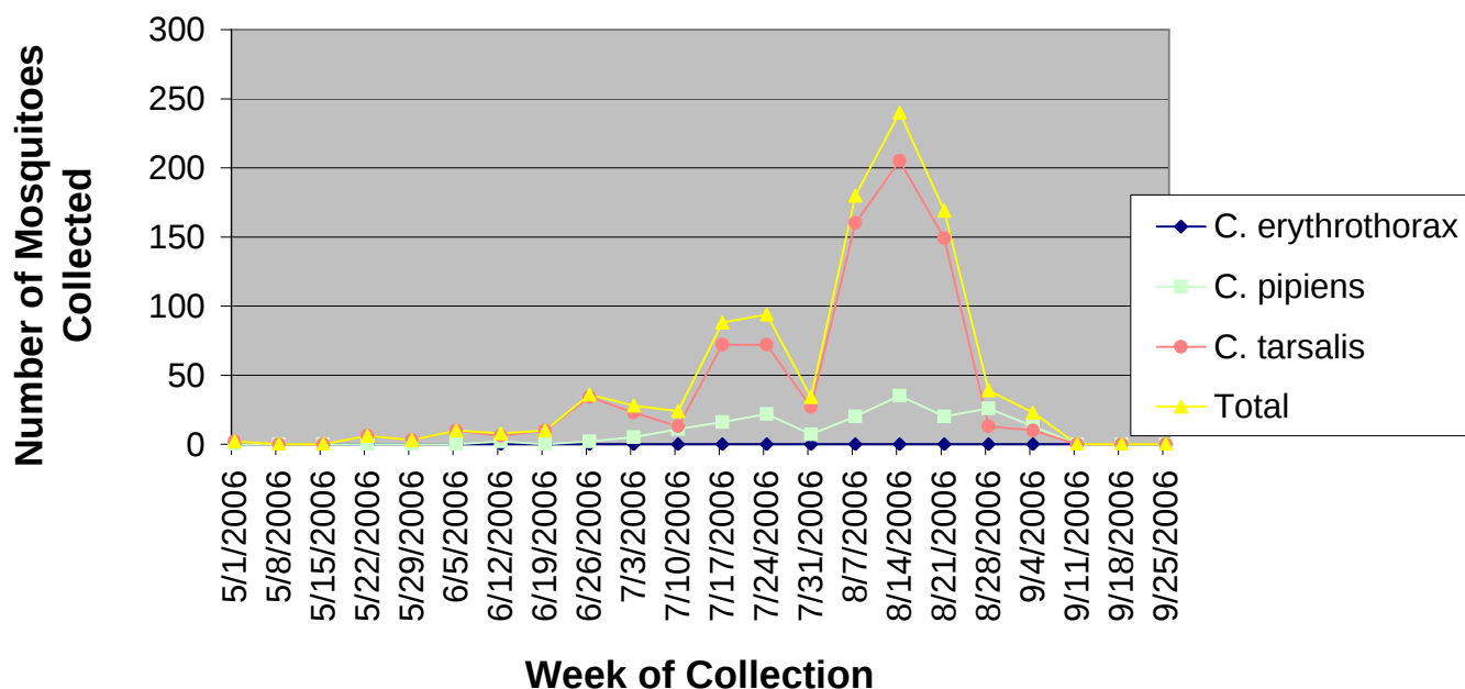
Number of Culex Mosquitoes Collected Larimer County Sentinel Site, 2006
