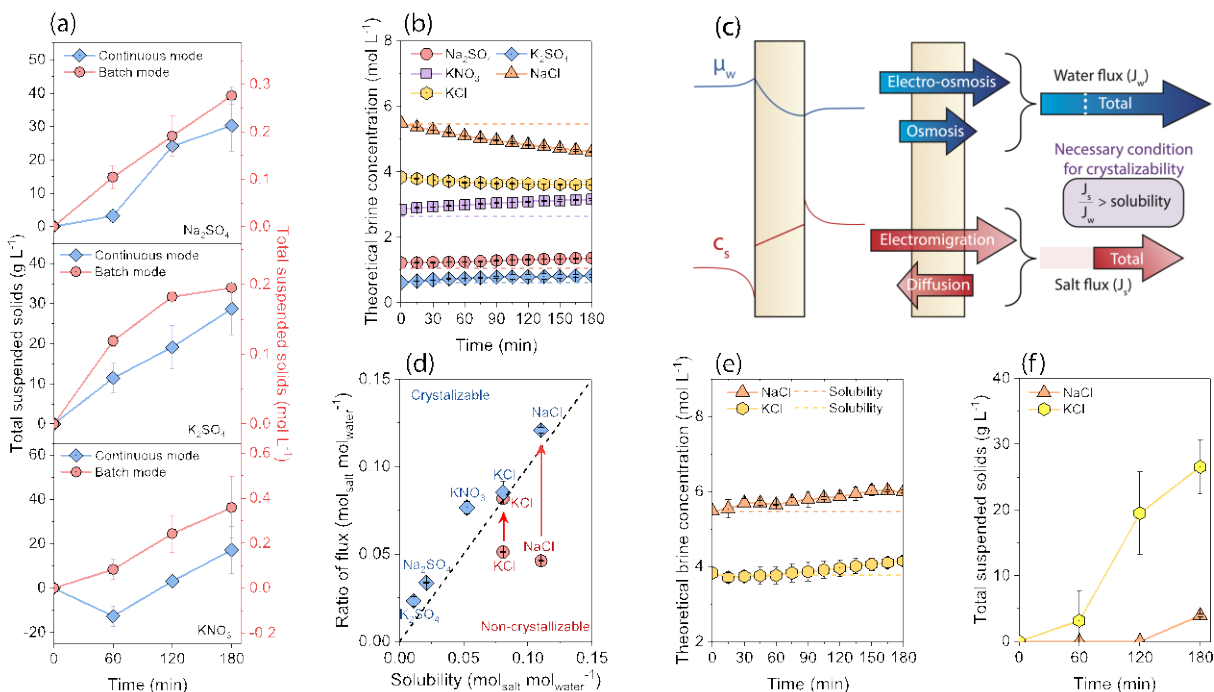
Figure 2. Crystallization of different salts in EDC. (a) Total suspended solids (TSS) production rates of \text{Na}_2\text{SO}_4 , \text{K}_2\text{SO}_4 and \text{KNO}_3 with continuous and batch modes. The ED cell configured with 5 pairs of the standard ion exchange membranes (IEMs). The applied current density was 40 \text{ mA cm}^{-2} . The initial diluate was 4 L of 0.6 M of each salt. The initial brine was 1 L of saturated solution of the respective salt (at 20^\circ\text{C} ). (b) Theoretical brine concentration, i.e., TDS plus TSS (if any), for five different salts. (c) Schematic illustration of salt crystallization mechanism in the EDC system. (d) Molar ratio of salt to water as calculated from the salt solubility at 18^\circ\text{C} (x axis) as compared to the ratio of salt flux to water flux in continuous mode (y axis). Blue rhombuses represent successful crystallization whereas red circles represent unsuccessful crystallization. (e) Theoretical brine concentration and (f) TSS for \text{NaCl} and \text{KCl} as a function of operation time with low-water-uptake IEMs and different operating conditions.
