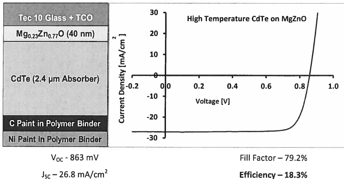
Figure 2: Device Structure for 18.3% efficiency device and the JV curve (J in mA/sq. cm. on the y-axis and volts on the x-axis).
