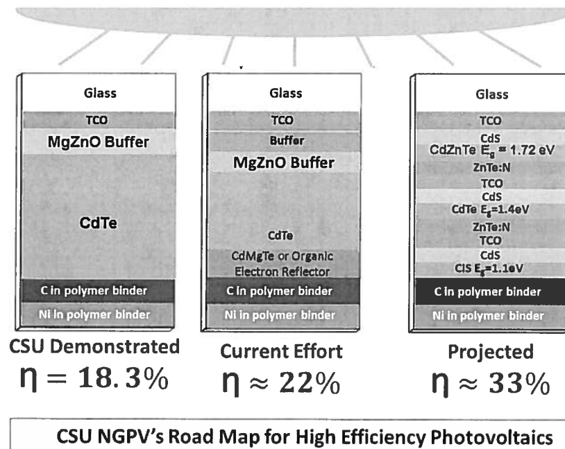
Figure 1: Efficiency Roadmap for CdTe Photovoltaics at CSU
