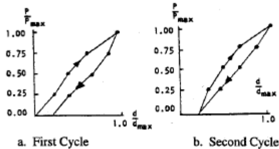
Figure 1. Static Load Test Load-Deflection Curves
