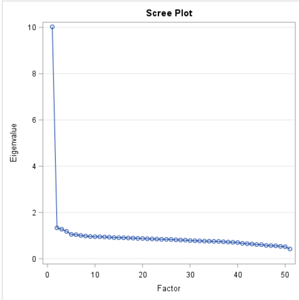
Figure 16. Grade 4 Social Studies Scree Plot
