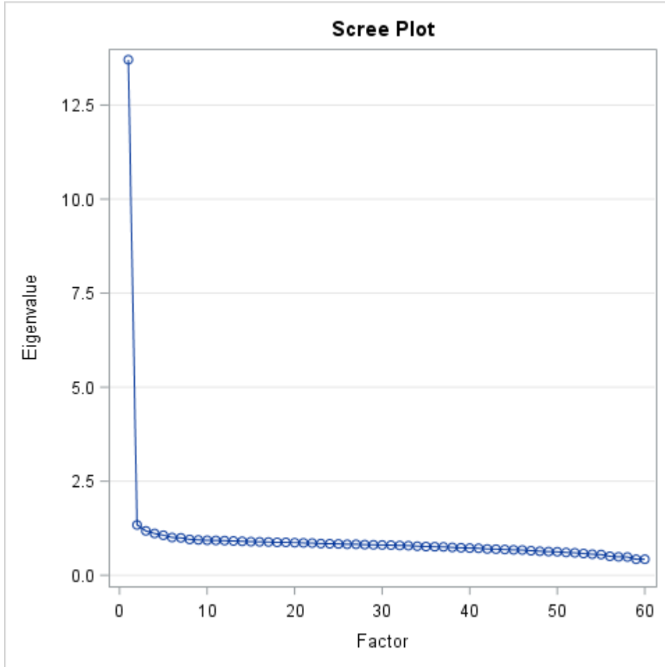
Figure 19. Grade 8 Science Scree Plot
