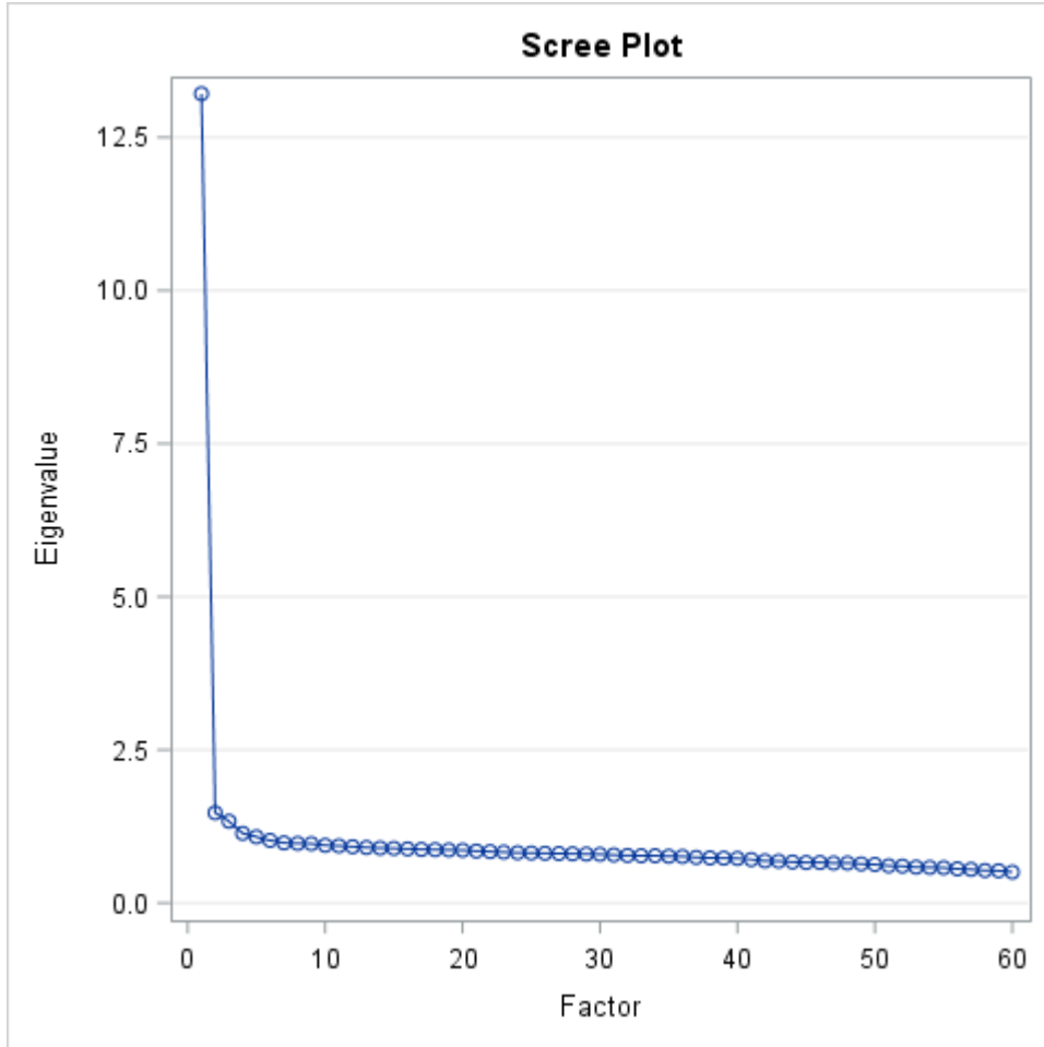
Figure 20. High School Science Scree Plot
