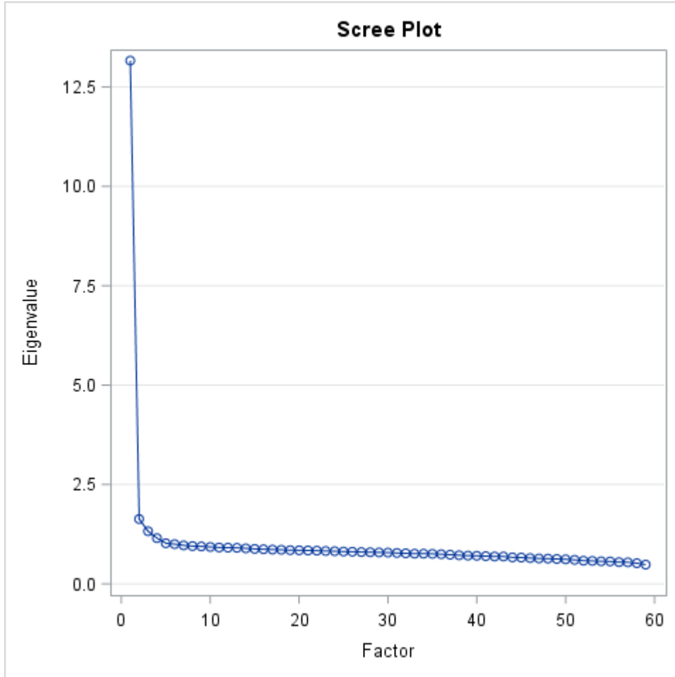
Figure 17. Grade 5 Science Scree Plot
