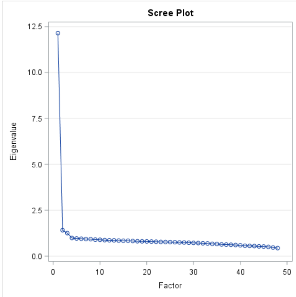
Figure 18. Grade 7 Social Studies Scree Plot
