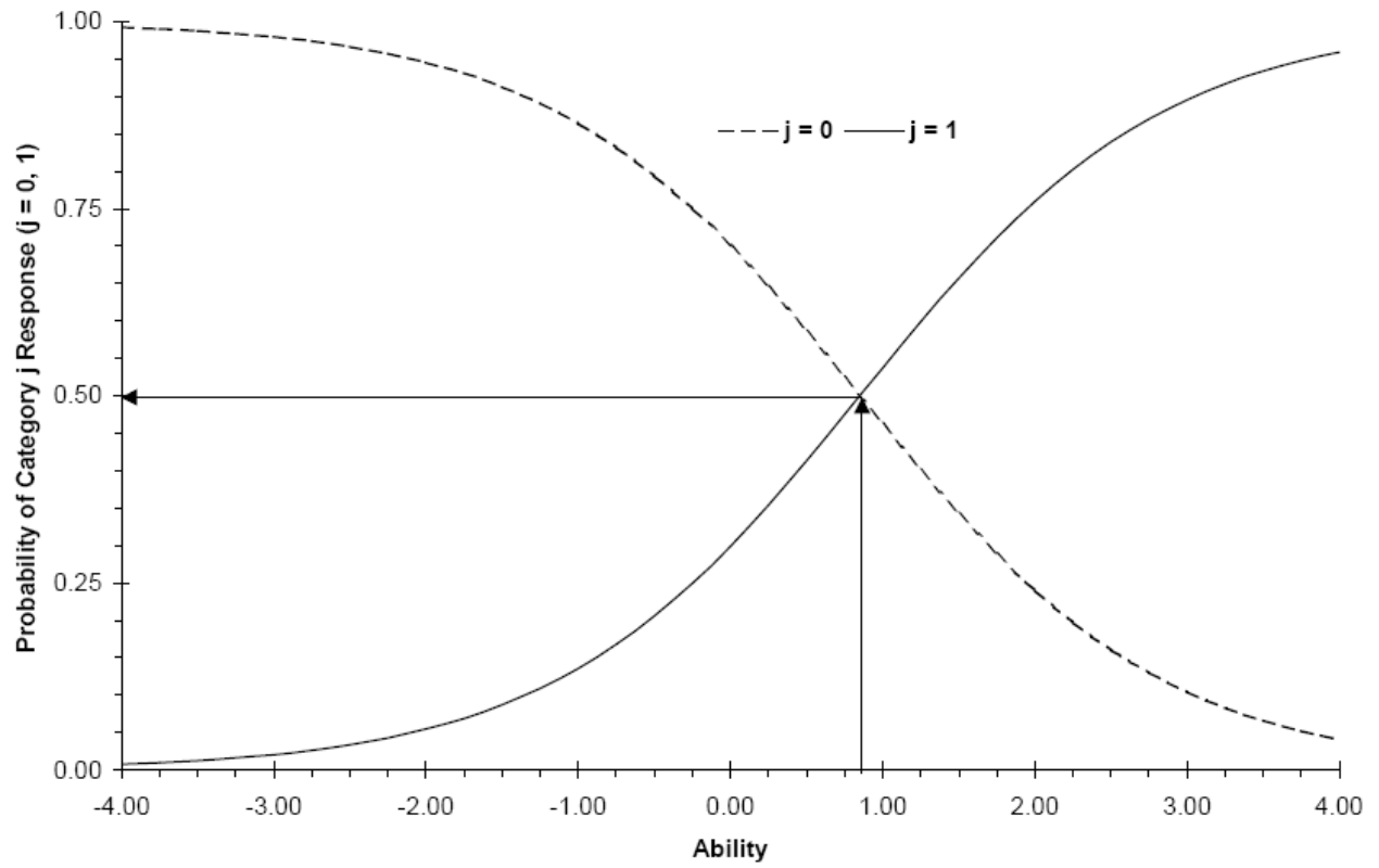
Figure 7. Sample 2PL Item Response Curves
