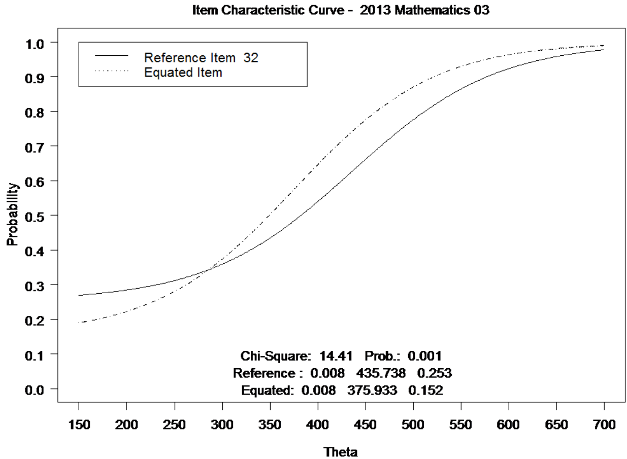
Figure 2. Item Characteristic Curves for Mathematics Grade 3 Anchor Item 32 Unanchored from the Equating of the Operational Test
