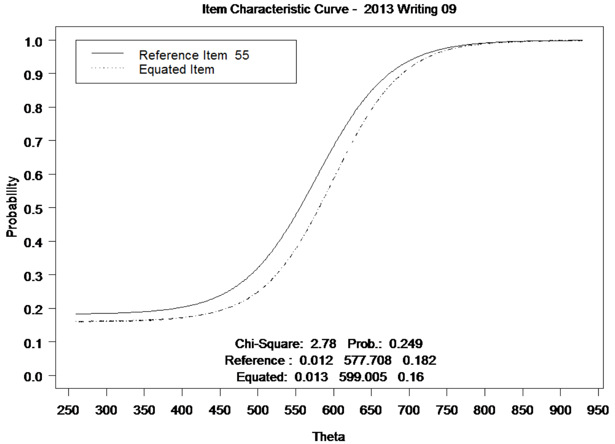
Figure 1. Item Characteristic Curves for Writing Grade 9 Anchor Item 55 Unanchored from the Equating of the Operational Test
