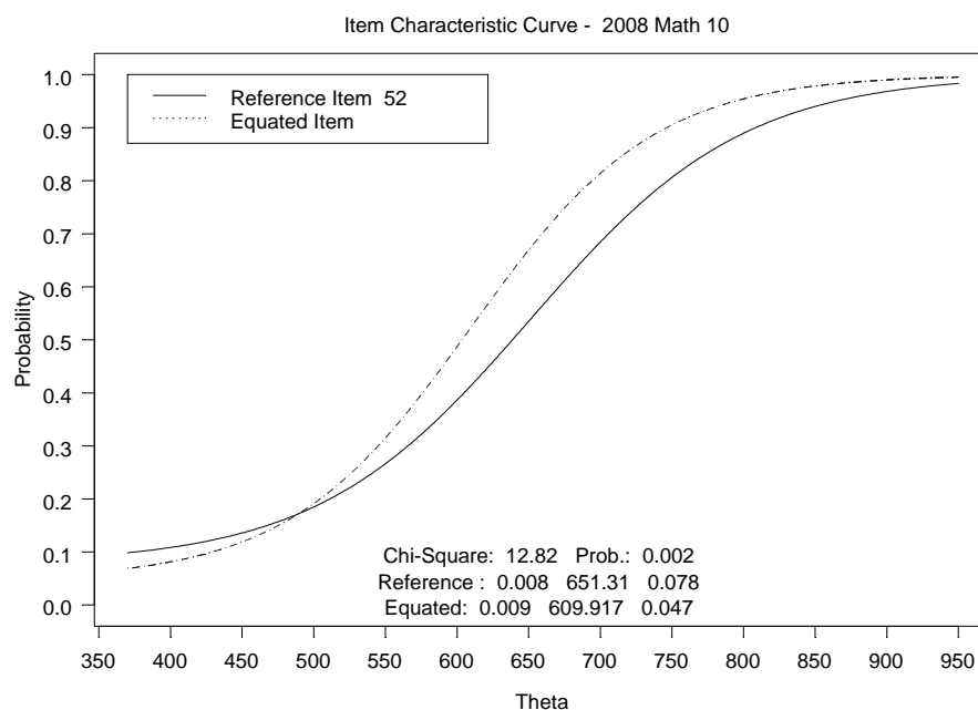
Figure 1. Item Characteristic Curves for Mathematics Grade 10 Anchor Item 52 Unanchored from the Equating of the Operational Test
